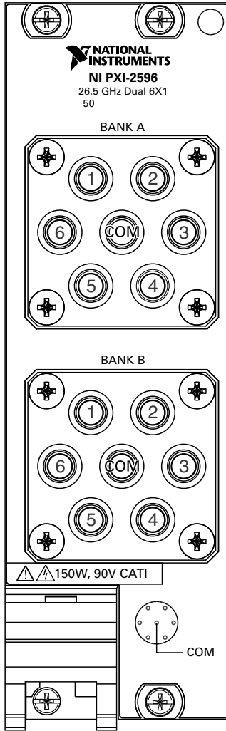
Figure 4. PXI-2596 Front Panel
