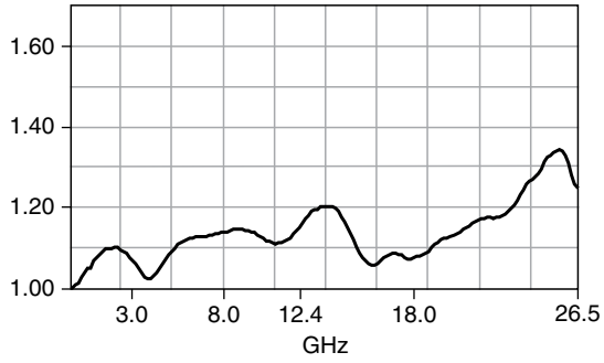
Figure 2. VSWR, Typical
